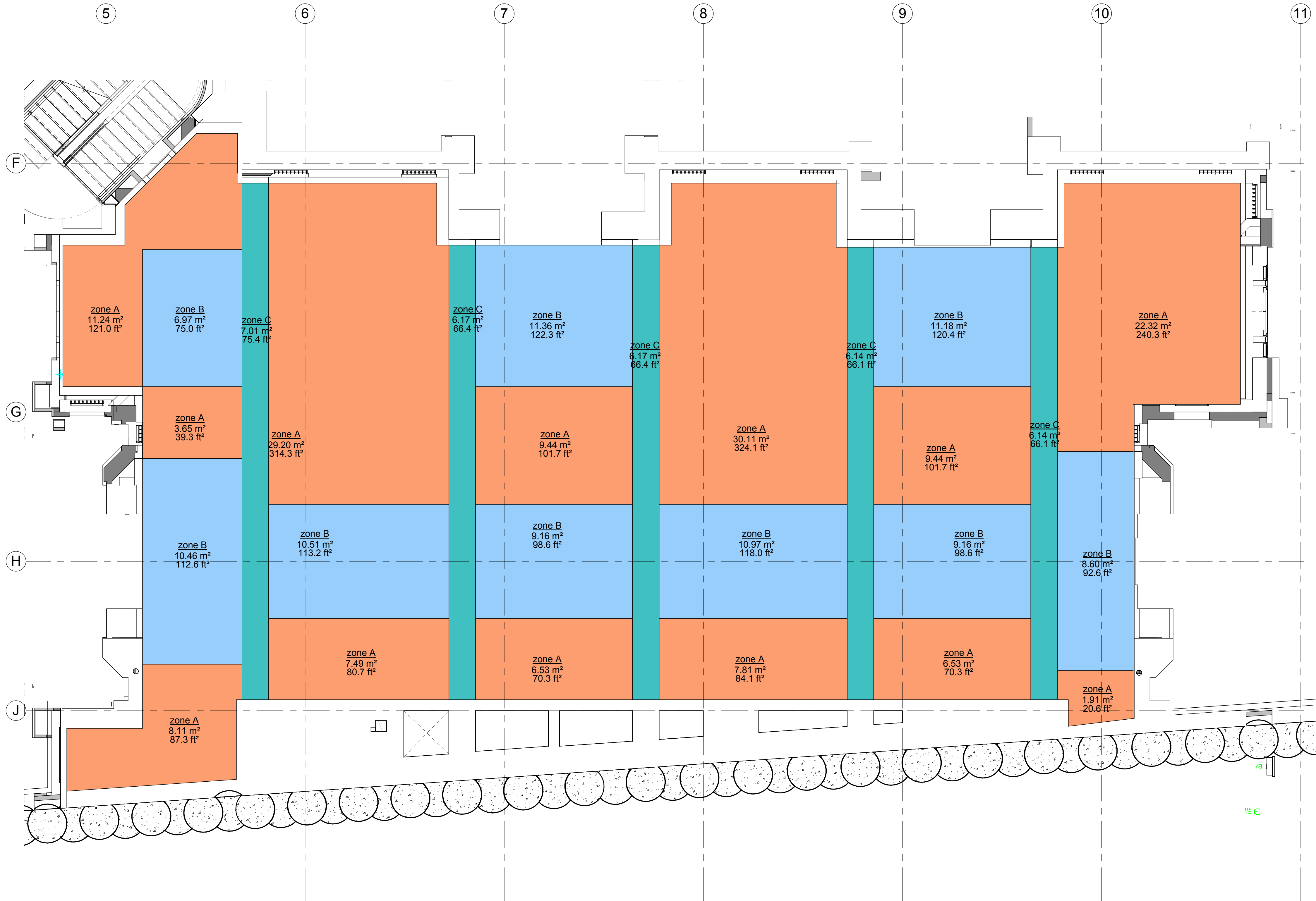
1 SK-226 - Garden insulation thickness 1 : 50
